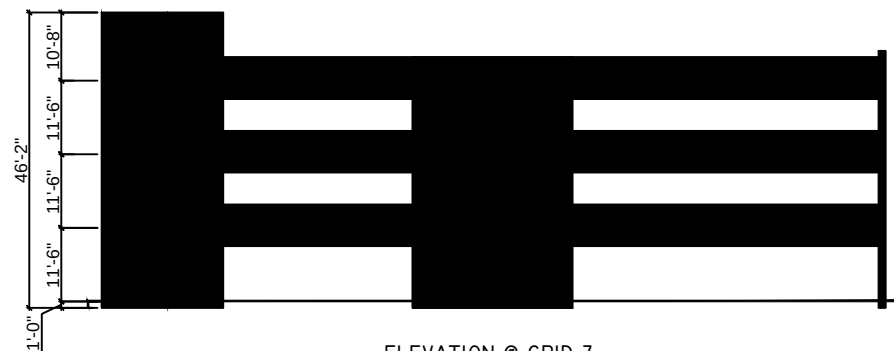
ELEVATION @ GRID 7 (EAST ELEVATION)
